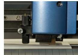
Onboard optical system locates registration marks on previously printed material for accurate print-and-cut applications.
